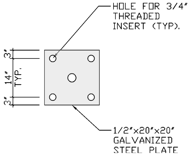
CONNECTION PLATE - WATERFRONT PARK
