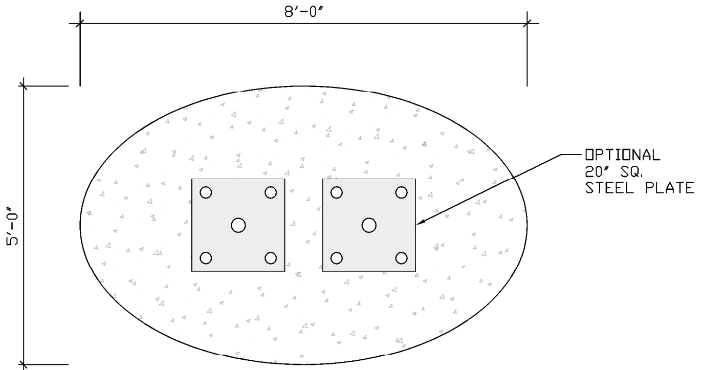
PLAN - WATERFRONT PARK PEDESTAL
