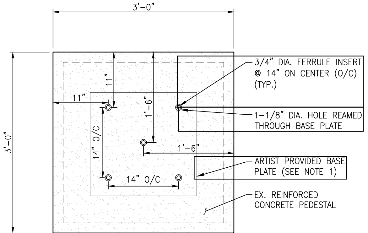
PLAN VIEW
