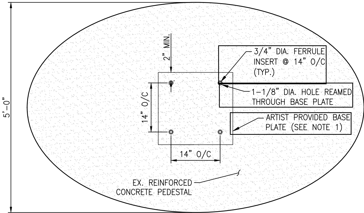
PLAN VIEW
