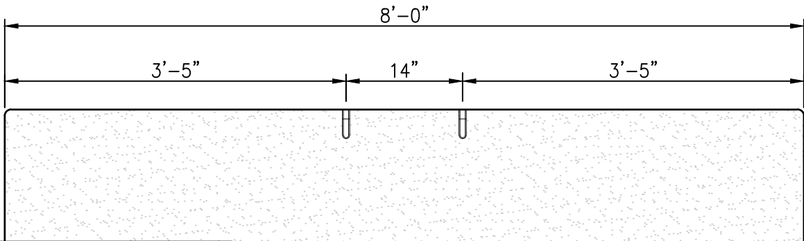
EX. FINISHED GRADE
